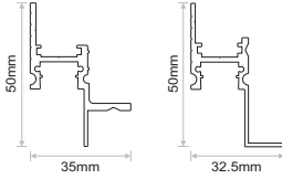
LINART C (Ceiling)
